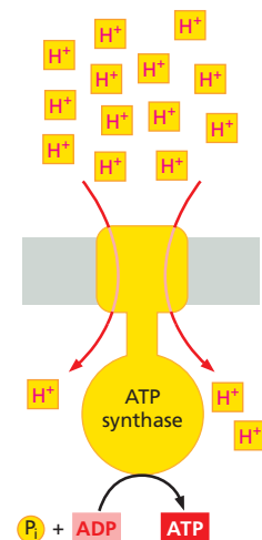
Figure 14–3 Stage 2 of chemiosmotic coupling. An ATP synthase (yellow) embedded in the lipid bilayer of a membrane harnesses the electrochemical proton gradient across the membrane, using it as a local energy store to drive ATP synthesis. The red arrows show the direction of proton movement through the ATP synthase.
