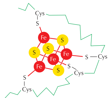
Figure 14–16 The structure of an iron-sulfur cluster. These dark brown clusters consist either of four iron and four sulfur atoms, as shown here, or of two irons and two sulfurs linked to cysteines in the polypeptide chain via covalent sulfur bridges, or to histidines. Although they contain several iron atoms, each iron-sulfur cluster can carry only one electron at a time. Nine different iron-sulfur clusters participate in electron transport in the respiratory chain.
