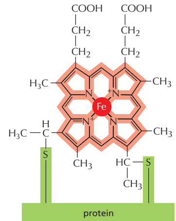
Figure 14–15 The structure of the heme group attached covalently to cytochrome c. The porphyrin ring of the heme is shown in red. There are six different cytochromes in the respiratory chain. Because the hemes in different cytochromes have slightly different structures and are kept in different local environments by their respective proteins, each has a different affinity for an electron, and a slightly different spectroscopic signature.
