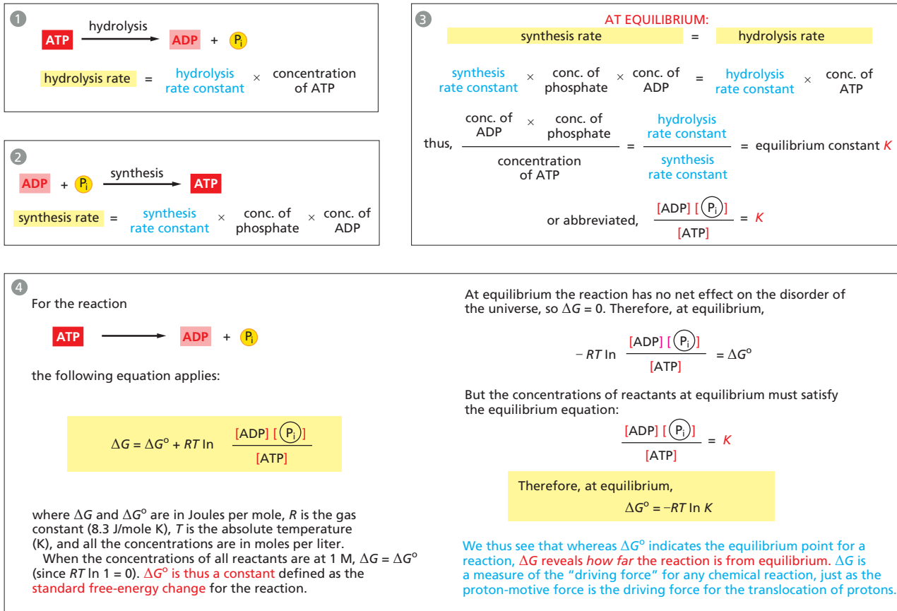
Figure 14–29 The basic relationship between free-energy changes and equilibrium in the ATP hydrolysis reaction.
