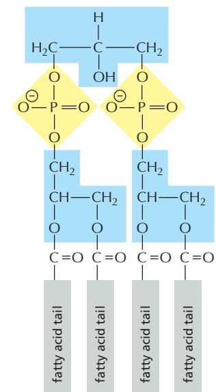
Figure 14-11 The structure of cardiolipin . Cardiolipin consists of two covalently linked phospholipid units, with a total of four rather than the usual two fatty acid chains (see Figure 10-3). Cardiolipin is only produced in the mitochondrial inner membrane, where it interacts closely with membrane proteins involved in oxidative phosphorylation and ATP transport. In cristae, its two juxtaposed phosphate groups may act as a local proton trap on the membrane surface.
