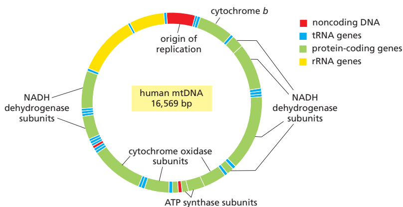
Figure 14–65 The organization of the human mitochondrial genome. The human mitochondrial genome of \approx 16,600 nucleotide pairs contains 2 rRNA genes, 22 tRNA genes, and 13 protein-coding sequences. There are two transcriptional promoters, one for each strand of the mitochondrial DNA (mtDNA). The DNAs of many other animal mitochondrial genomes have been completely sequenced. Most of these animal mitochondrial DNAs encode precisely the same genes as humans, with the gene order being identical for animals ranging from fish to mammals.
