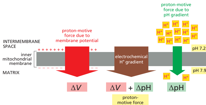
Figure 14-14 The electrochemical proton gradient across the inner mitochondrial membrane. This gradient is composed of a large force due to the membrane potential ( \Delta V ) and a smaller force due to the \text{H}^+ concentration gradient—that is, the pH gradient ( \Delta\text{pH} ). Both forces combine to generate the proton-motive force, which pulls \text{H}^+ back into the mitochondrial matrix. The exact relationship between these forces is expressed by the Nernst equation (see Panel 11-1, p. 616).
