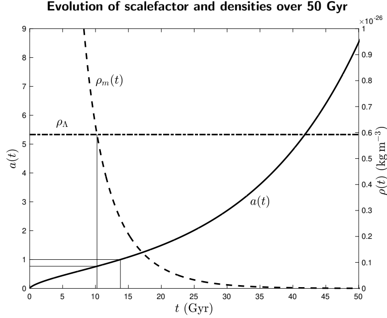
Figure 13.4 The scale factor a (solid), the vacuum density \rho_\Lambda (dotdash), and the matter density \rho_m (dashed) are plotted as functions of the time (13.325) in Gyr. The era of matter ends at t = 10.228 Gyr (first vertical line) when the two densities are equal to 5.9238 \times 10^{-27} \text{kg m}^{-3} and a = 0.7672 . The present time t_0 is 13.787 Gyr (second vertical line) at which a(t) = 1 .
