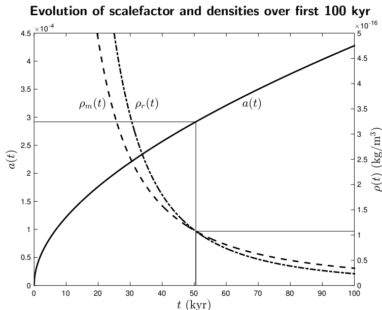
Figure 13.3 The Planck-collaboration scale factor a (solid), radiation density \rho_r (dotdash), and matter density \rho_m (dashed) are plotted as functions of the time (13.325) in kyr. The era of radiation ends at t = 50,506 years when the two densities are equal to 1.0751 \times 10^{-16} \text{ kg/m}^3 , a = 2.919 \times 10^{-4} , and z = 3425 .
