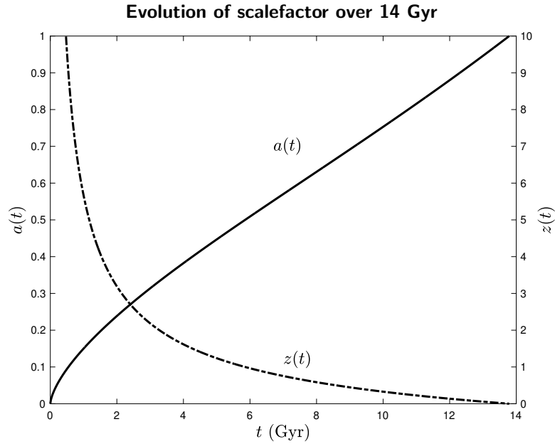
Figure 13.2 The scale factor a(t) (solid, left axis) and redshift z(t) (dotdash, right axis) are plotted against the time (13.325) in Gyr. This chapter's Fortran, Matlab, and Mathematica scripts are in Tensors_and_general_relativity at github.com/kevinecahill .
